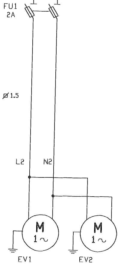
VENTILATORI ARMADIO 28/29W 220/230VAC
